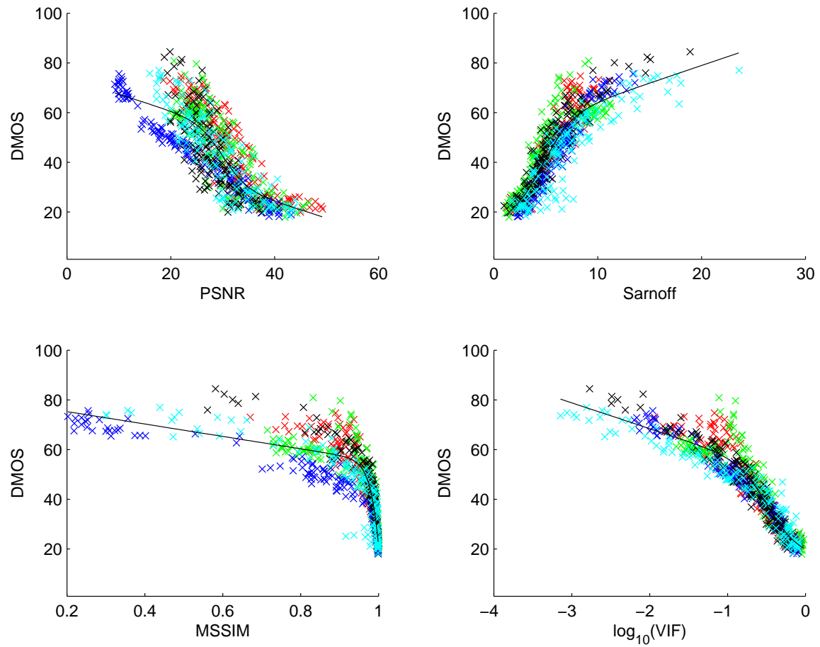
Fig. 8. Scatter plots for the four objective quality criteria: PSNR, Sarnoff's JND-matrix, MSSIM, and \log_{10}(\text{VIF}) for VIF using horizontal/vertical orientations. The distortion types are: JPEG2000 (red), JPEG (green), white noise in RGB space (blue), Gaussian blur (black), and transmission errors in JPEG2000 stream over fast-fading Rayleigh channel (cyan).
