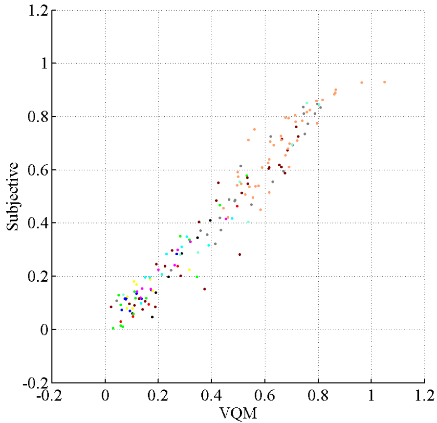
Figure 37. HRC subjective quality vs. HRC VQM_D .
