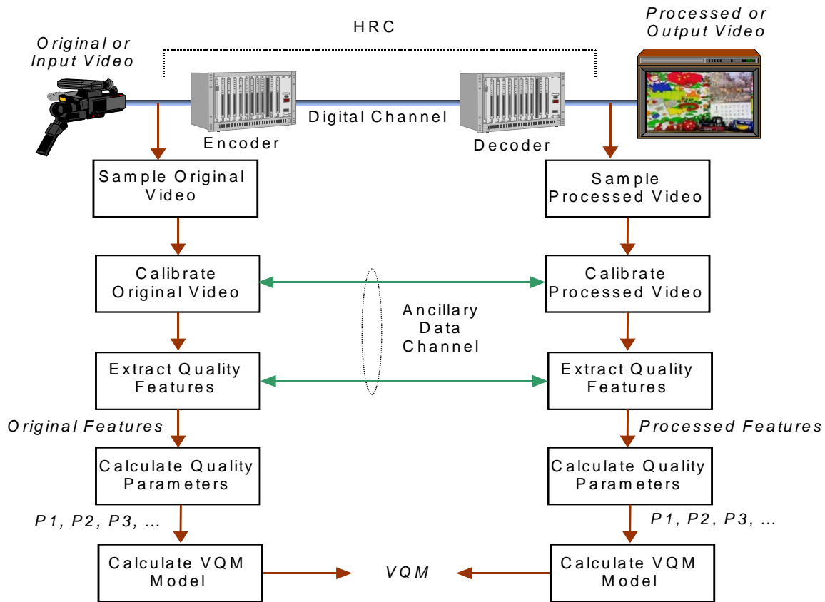
Figure 1. Steps required to compute VQM.
