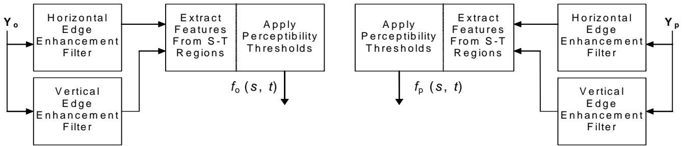
Figure 26. Overview of algorithm used to extract spatial gradient features.
