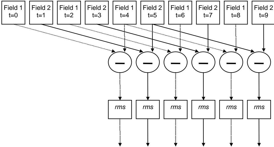
Figure 13. Diagram depicting the method of calculating TI4( t ).
