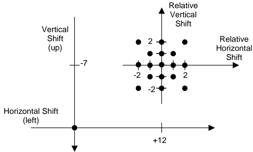
Figure 8. Spatial shifts considered by the fine search for the spatial shift.
