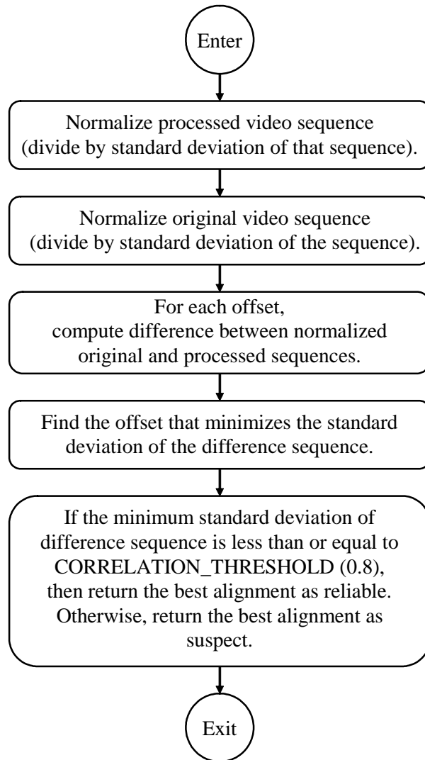
Figure 14. Correlation algorithm description.
