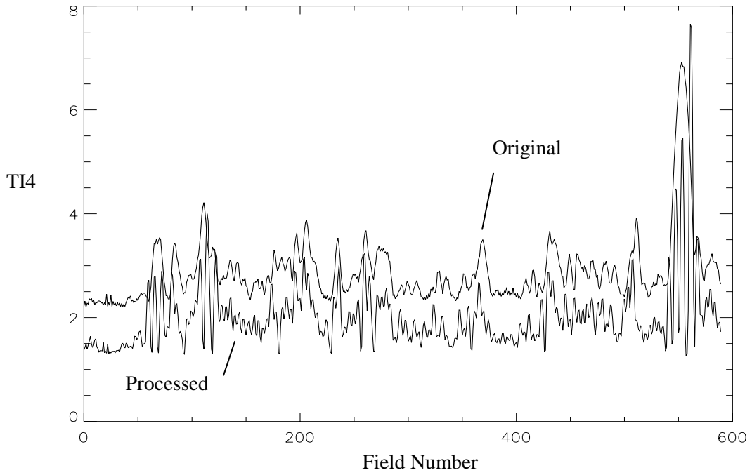
Figure 22. Original and processed feature TI4 for the scene vtc1nw and HRC 18, failed alignment.
