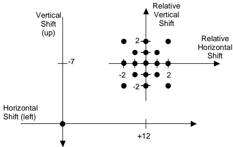
Figure 11. Spatial shifts considered by the fine search for the spatial shift.
