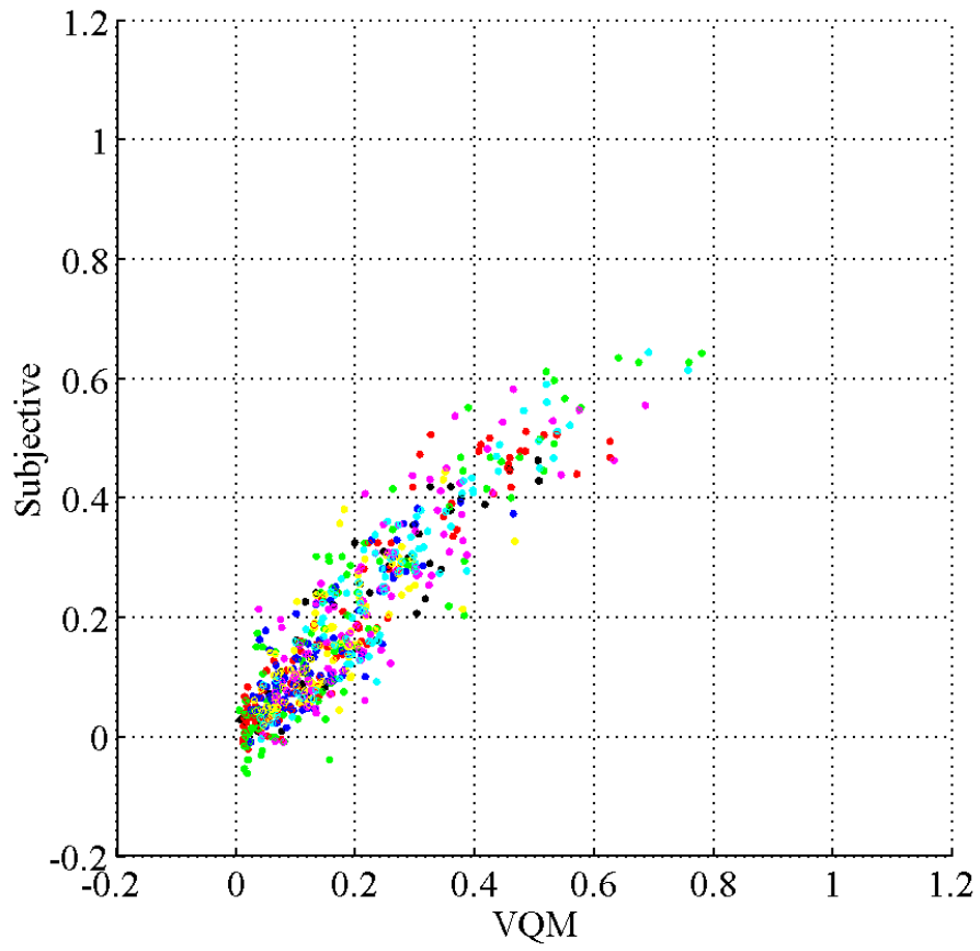
Figure 30. Clip subjective quality vs. clip VQM_T .
