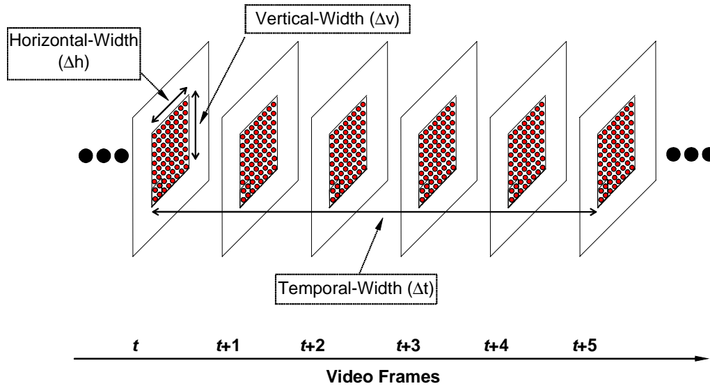
Figure 25. Example spatial-temporal (S-T) region size for extracting features.
