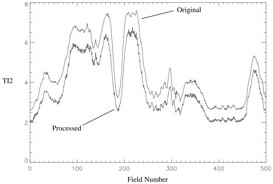
Figure 16. Aligned original and processed feature TI2 for the scene 5row1 and HRC 2.
