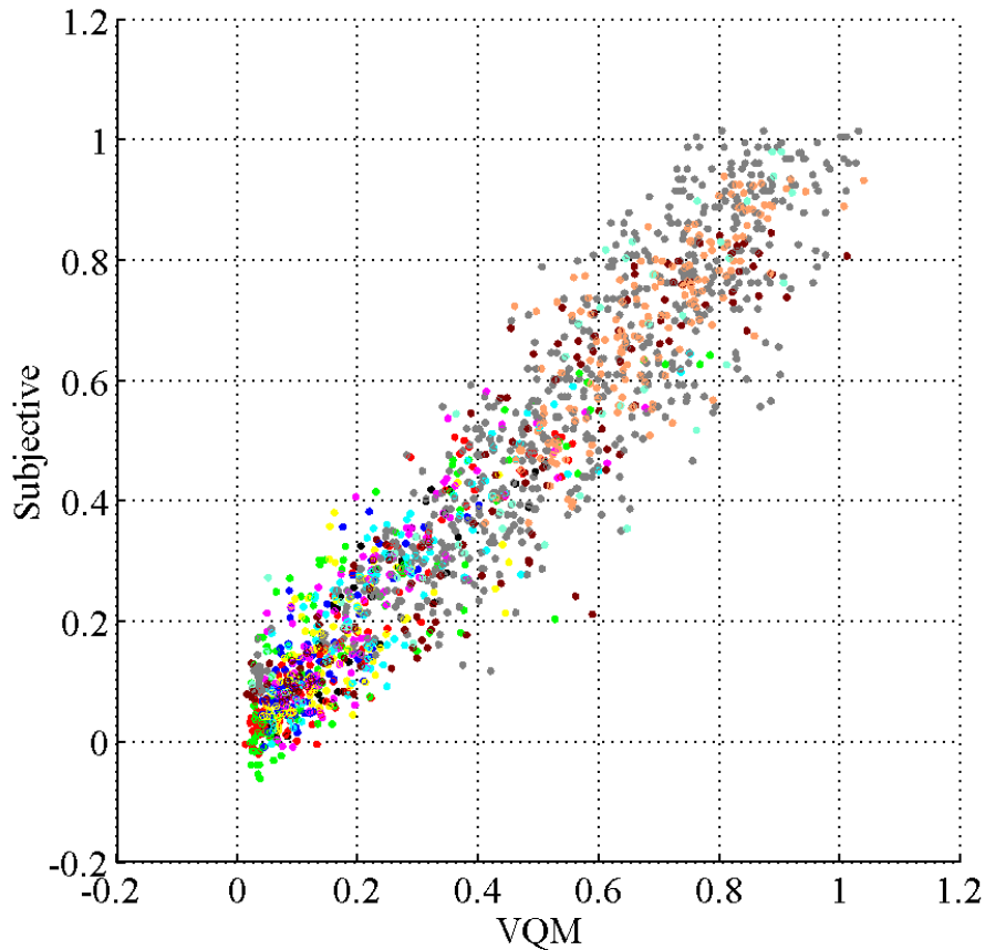
Figure 34. Clip subjective quality vs. clip VQM_G .
