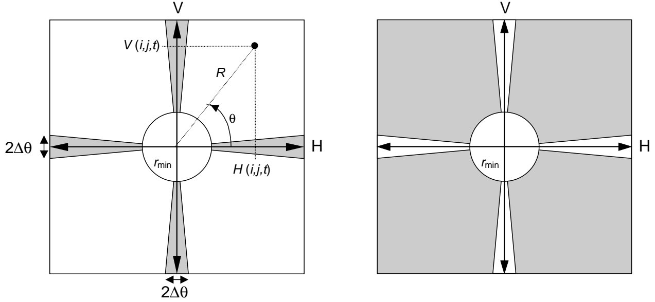
Figure 28. Division of horizontal (H) and vertical (V) spatial activity into HV (left) and \overline{HV} (right) distributions.
