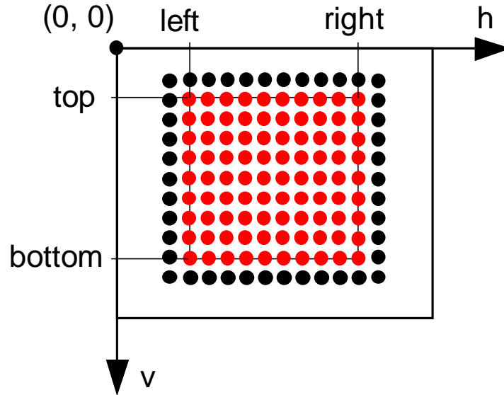
Figure 4. Rectangle coordinates for specifying image sub-regions.
