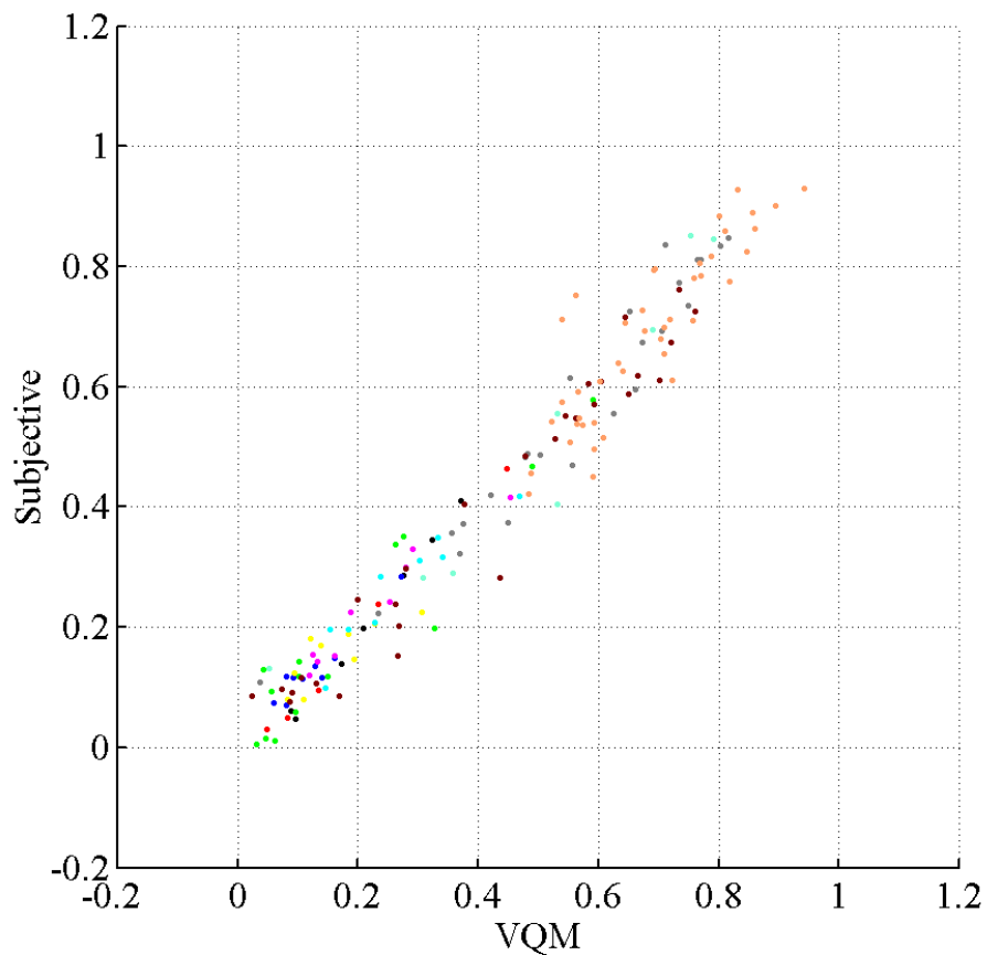
Figure 35. HRC subjective quality vs. HRC VQM_G .
