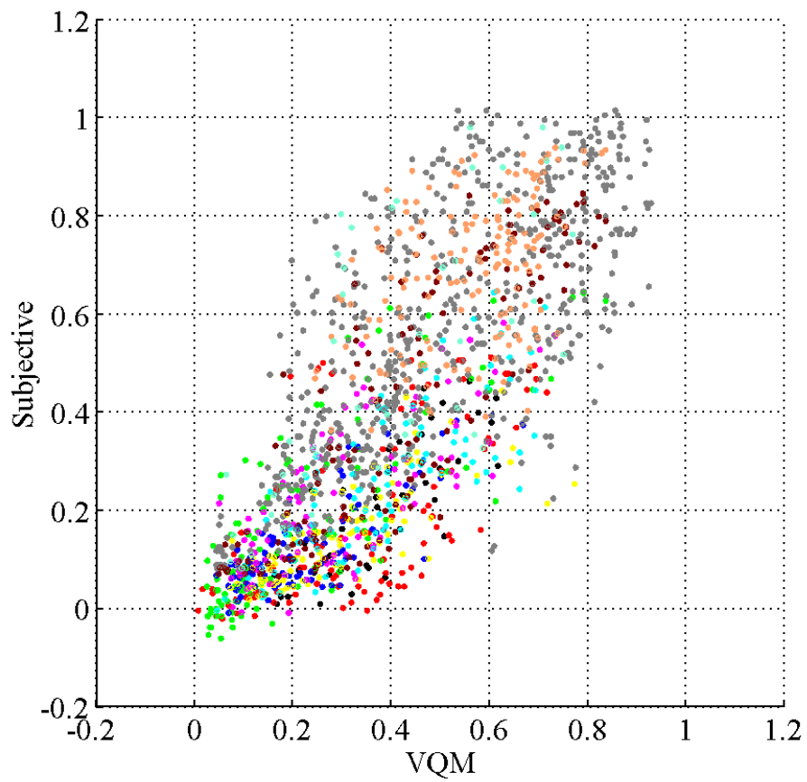
Figure 38. Clip subjective quality vs. clip VQM_p .
