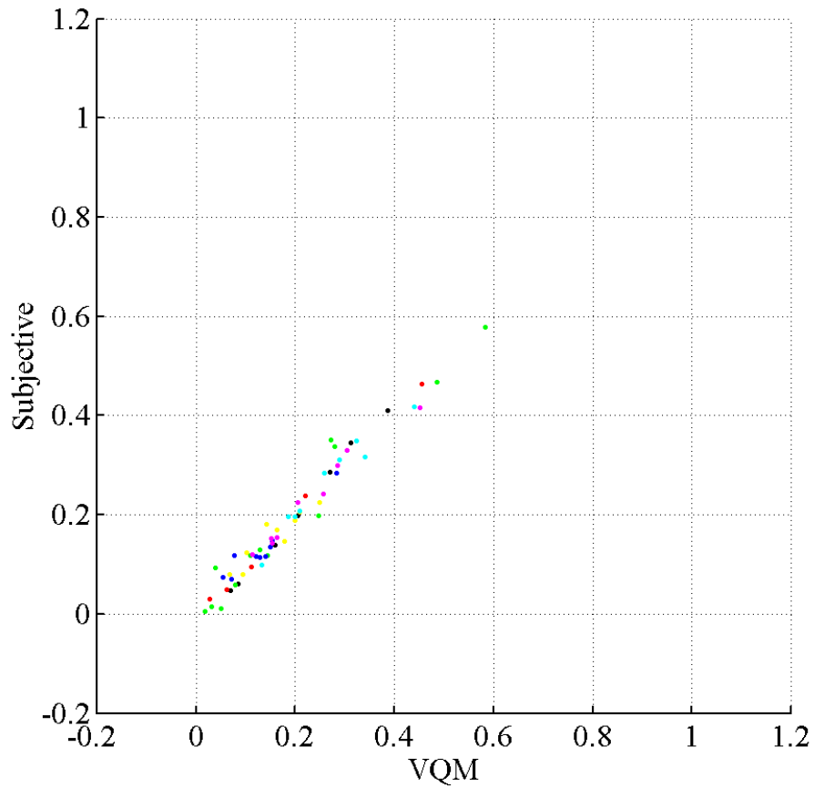
Figure 31. HRC subjective quality vs. HRC VQM T .
