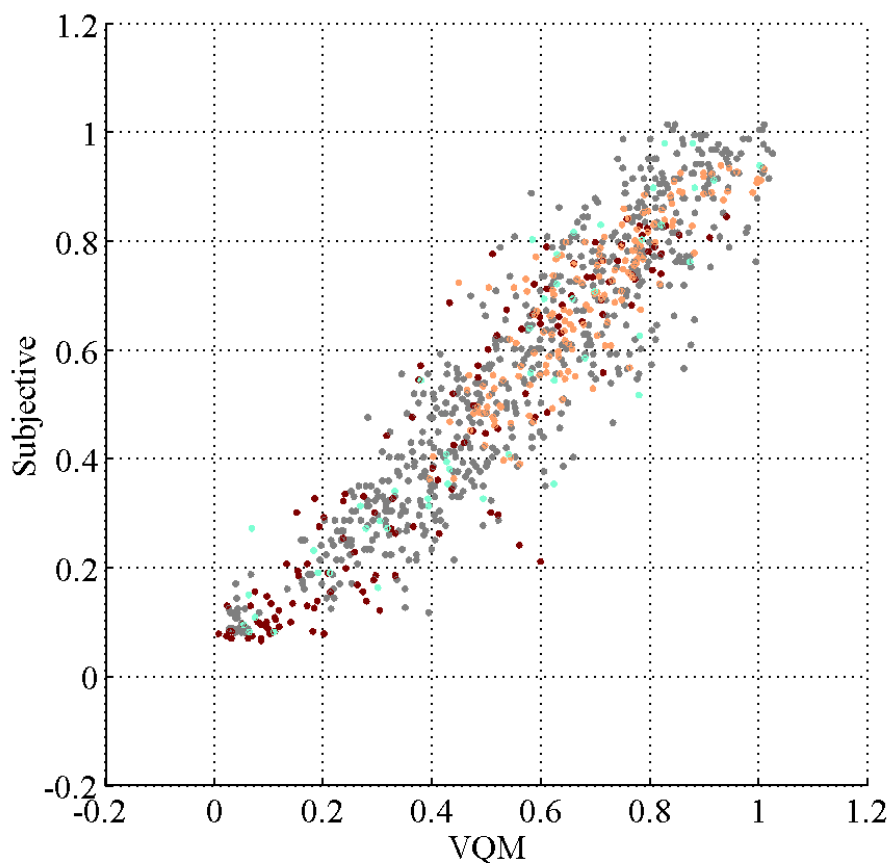
Figure 32. Clip subjective quality vs. clip VQM_V .
