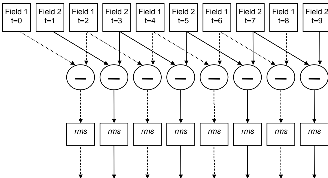
Figure 12. Diagram depicting the method of calculating TI2(t) .
