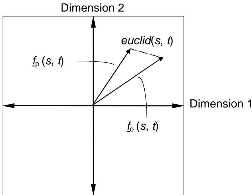
Figure 29. Illustration of the Euclidean distance euclid(s, t) for a two-dimensional feature vector.
