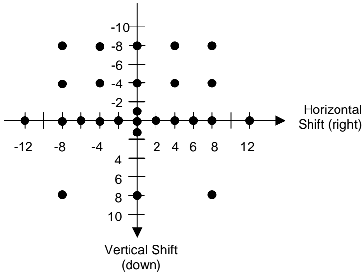
Figure 7. Spatial shifts considered by the broad search for the spatial shift.
