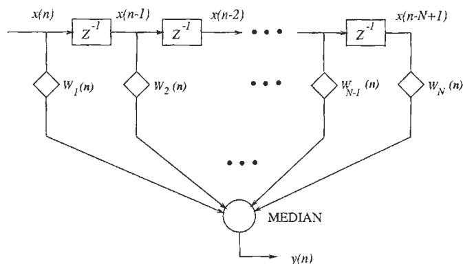
FIGURE 2 The weighted median smoothing operation.
