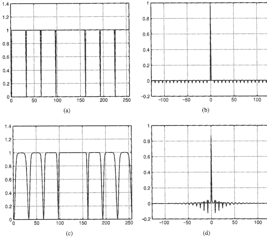
FIGURE 5 (a) |H_{\text{all}}(u, 0)| for direct implementation of the inverse filter; (c) |H_{\text{all}}(u, 0)| for the iterative implementation of the inverse filter; (b),(d) h_{\text{all}}(n, 0) corresponding to (a) and (c).
