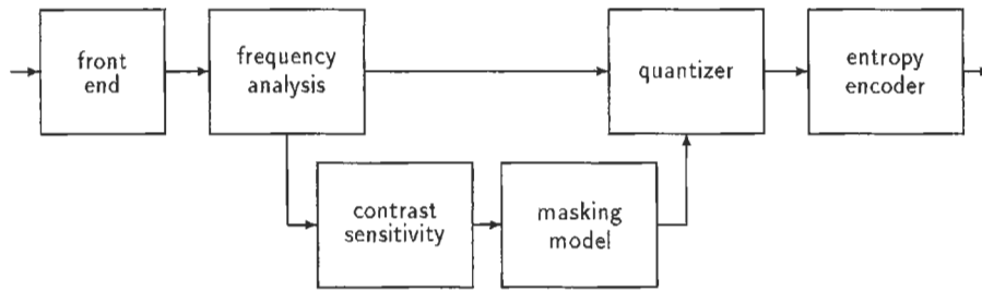
FIGURE 6 Perceptual coder.
