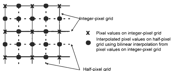
FIGURE 2 Half-pixel motion estimation.
