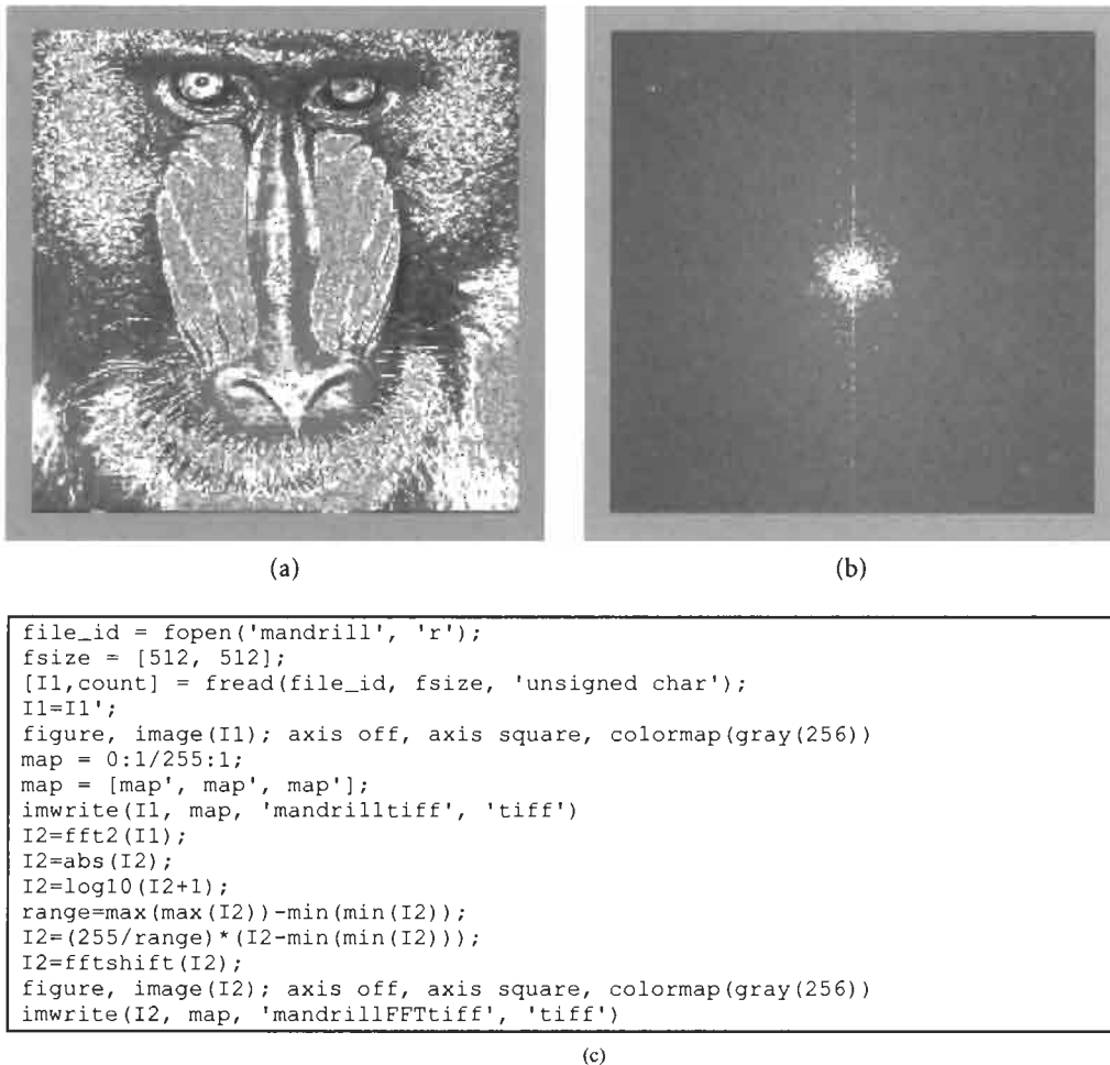
FIGURE 1 MATLAB example: (a) image, (b) FFT, and (c) code to display images, compute the FFT, and write out the TIFF images.
