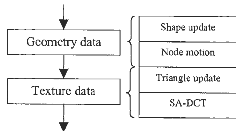
FIGURE 4 Overview of the intercoding mode syntax.
