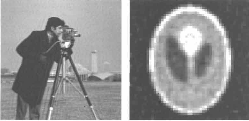
FIGURE 9 Brownian motion prior-based MAP solutions corresponding to the data in Figs. 1(b) (left) and 2(b) (right).
