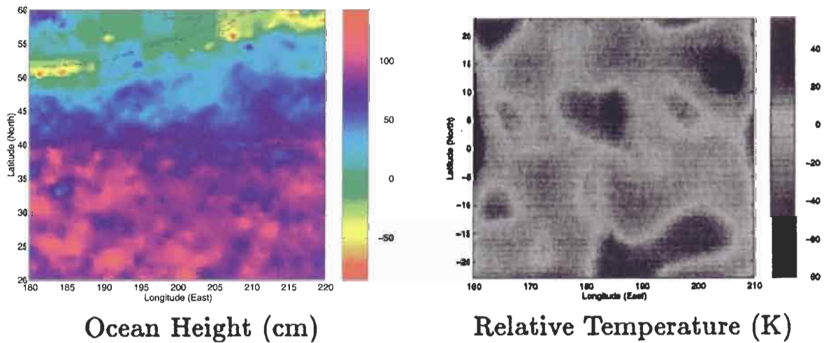
FIGURE 4.3.12 Multiscale estimation of remotely sensed fields: left, North-Pacific altimetry based on Topex/Poseidon data; right, equatorial Pacific temperature estimates based on in situ ship data.
