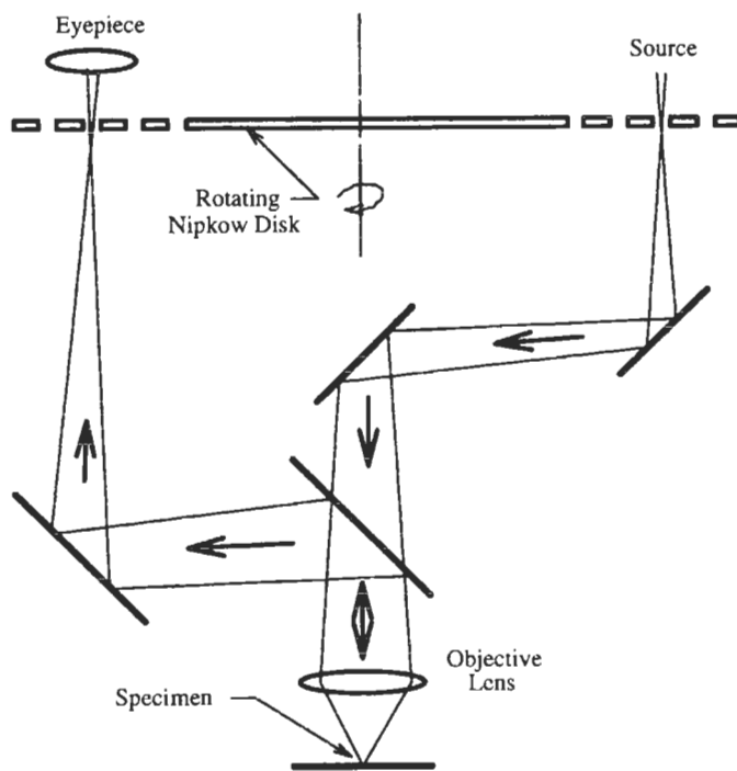
FIGURE 6 Diagram of the tandem scanning optical microscope.
