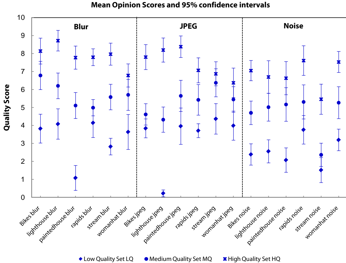
Figure 2 - Mean Opinion Scores for the stimuli in the dataset (cfr. Table I). Each panel in the graph corresponds to a given distortion type: i.e. Gaussian Blur (left), JPEG compression (center) and White Noise (Right). The different symbols in the graph correspond to different quality levels. Error bars indicate the 95% confidence interval of the MOS.
